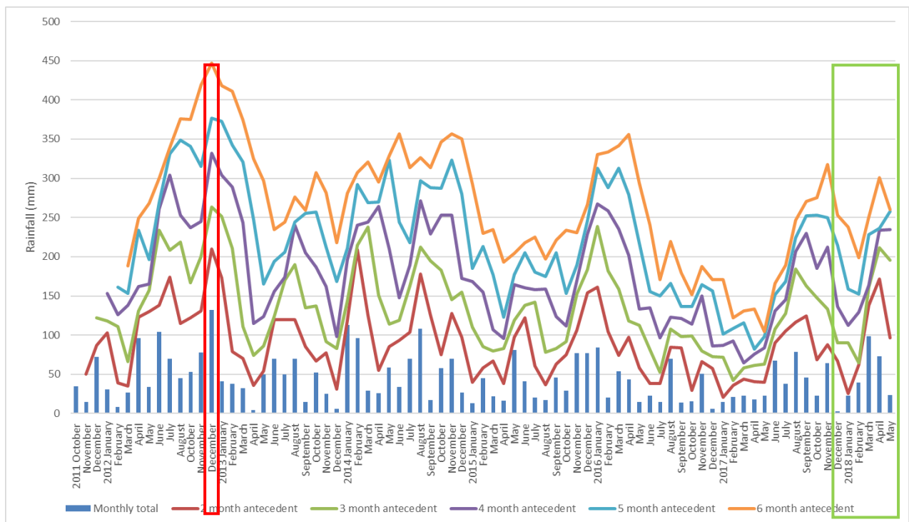
Figure 2.6. Monthly rainfall and two to six month antecedent totals (2011 to 2018). Ground movements were recorded at Scalby Mills during December 2012 (red box). Current monitoring period shown by green box.
