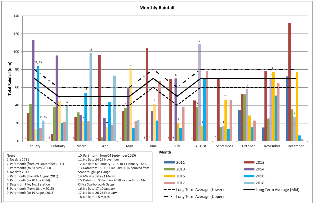
Figure 2.1 Comparison of monthly rainfall records (2011 to 2018).
