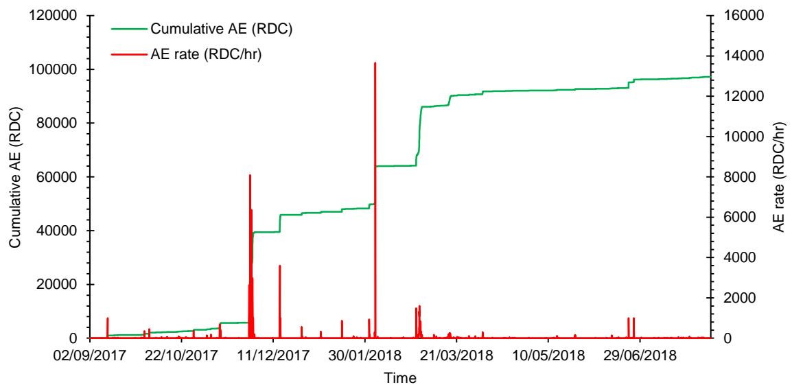
Figure 11.2 Cumulative AE (RDC) and AE rate (RDC/hr) time series at Flat Cliffs, Filey for the September 2017 to August 2018.
