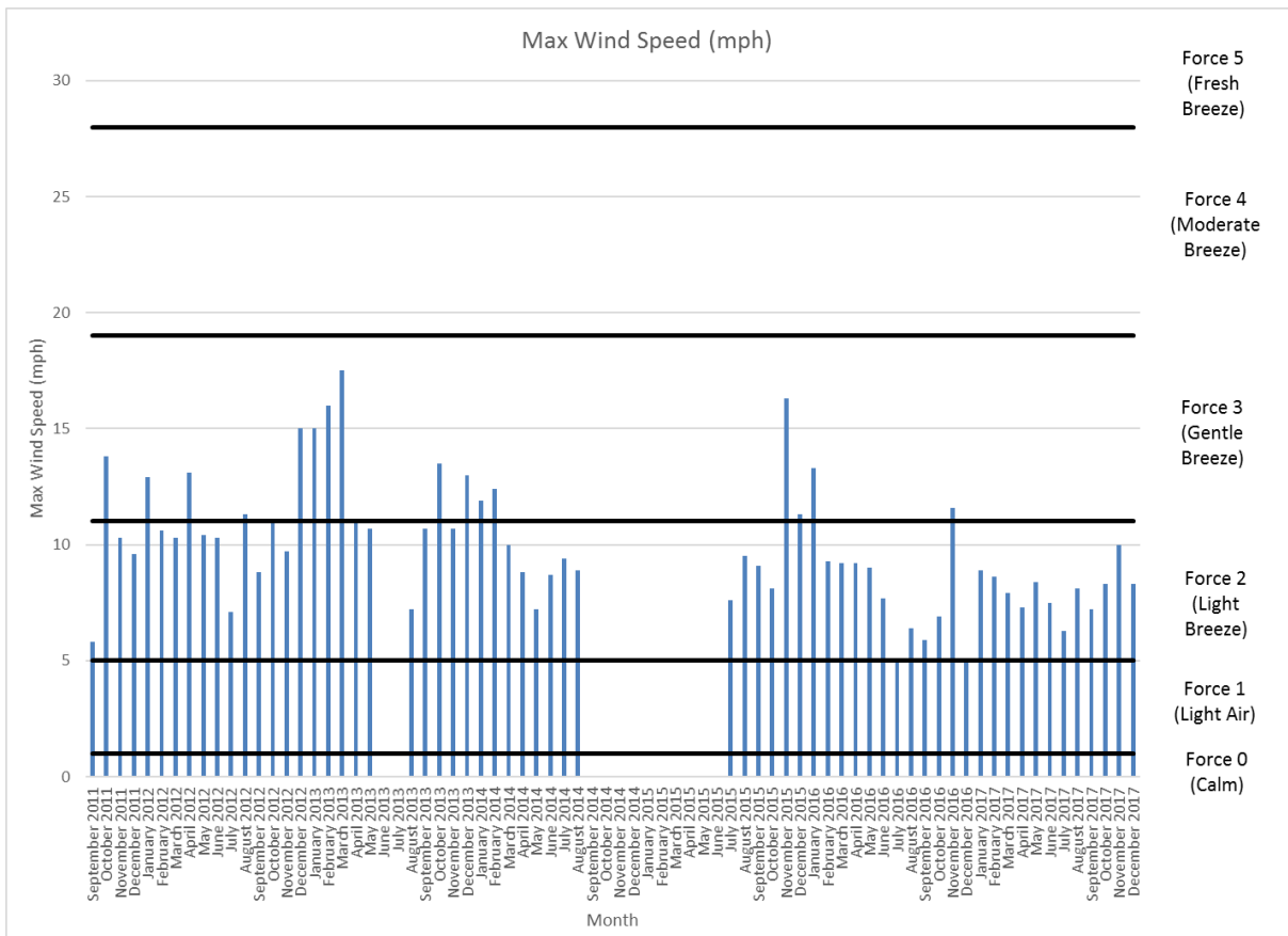
Figure 2.4 Maximum daily wind speed (2011 to 2017). Note there are no data for the current monitoring period.
