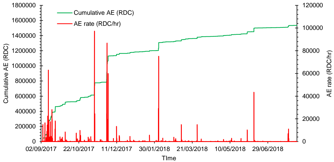
Figure 9.2. Cumulative AE (RDC) and AE rate (RDC/hr) time series at Scarborough Spa for the period September 2017 to August 2018.
