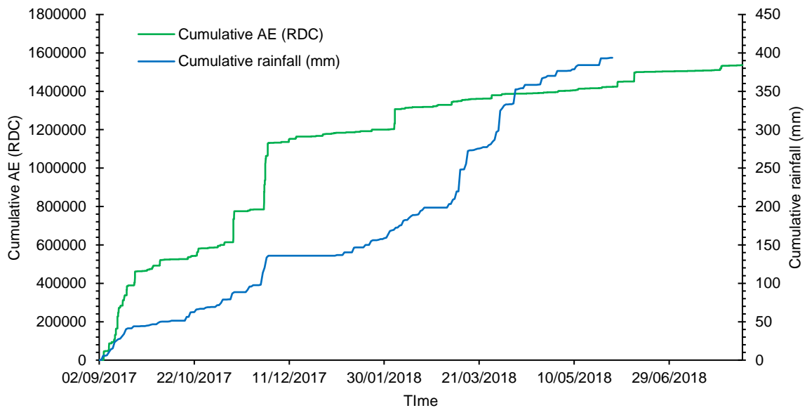
Figure 9.3. Cumulative AE (RDC) and cumulative rainfall time series at Scarborough Spa for the period September 2017 to August 2018.
